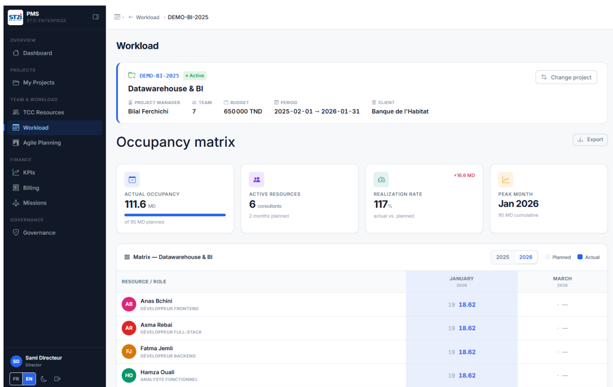
FIGURE 5.6 : Workload matrix interface
